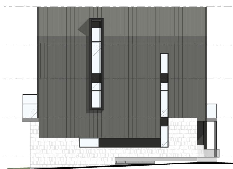
EAST ELEVATION
