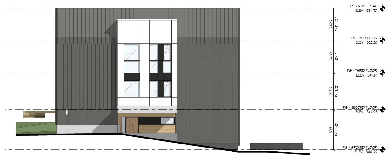
NORTH ELEVATION
