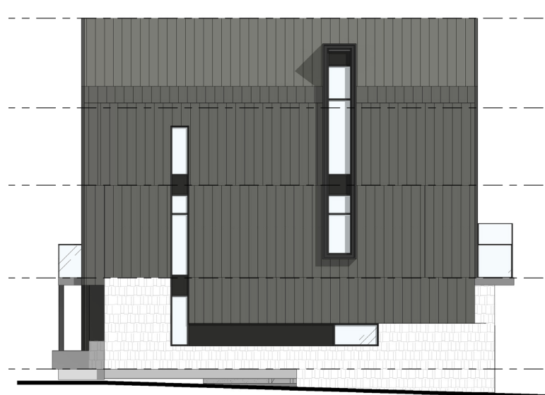
WEST ELEVATION
