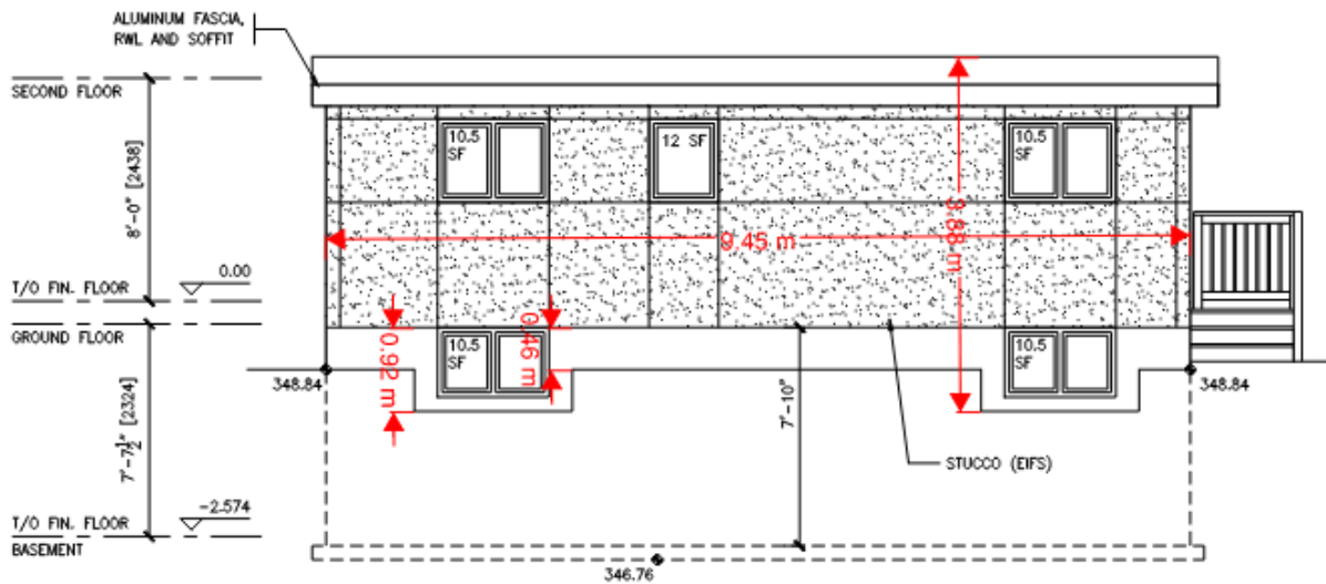
Figure E – Front Elevation of Proposed ADU (Detached)
