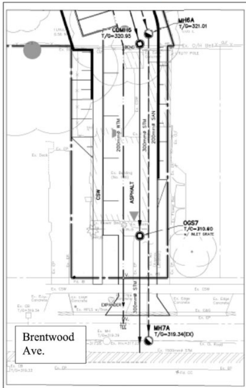
Figure 6 – Proposed Servicing through 136 Brentwood Avenue
