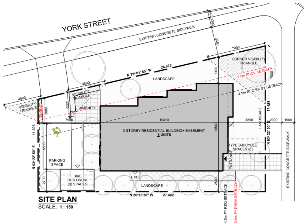
Figure 2: Site Plan
