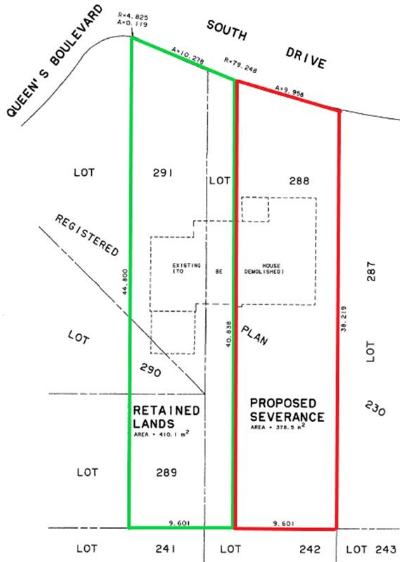
Figure 3: Severance sketch of two lots
