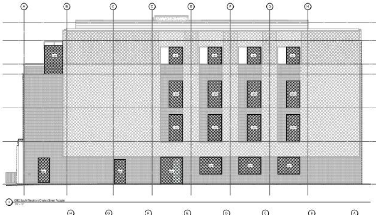
Elevation of wall face facing Charles St. E. showing proposed new openings
