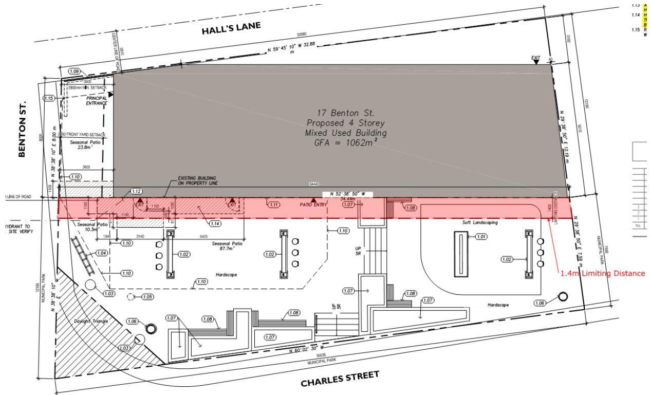
Site Plan – Existing Building at 17 Benton St., adjacent Oktoberfest Platz
