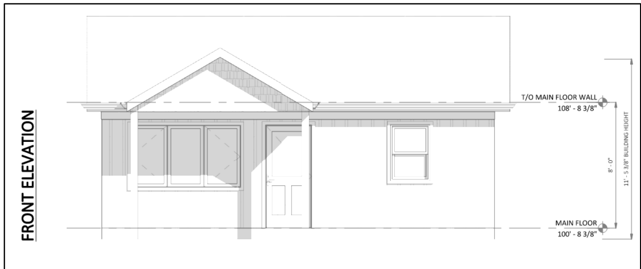
Figure 4 - Elevation drawing of the proposed ADU (Detached)
