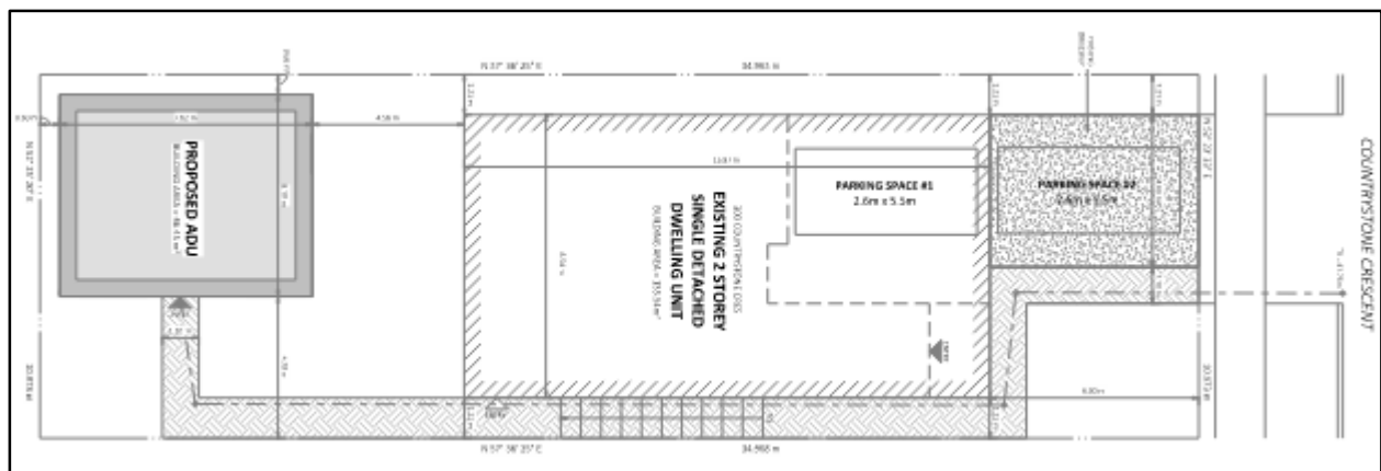
Figure 3 Site plan drawing showing the proposed ADU detached
